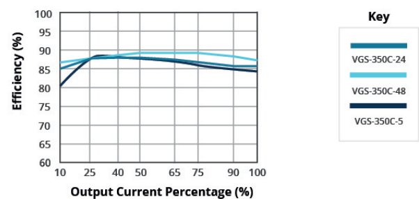
EFFICIENCY VS OUTPUT LOAD (VIN = 230 VAC)
