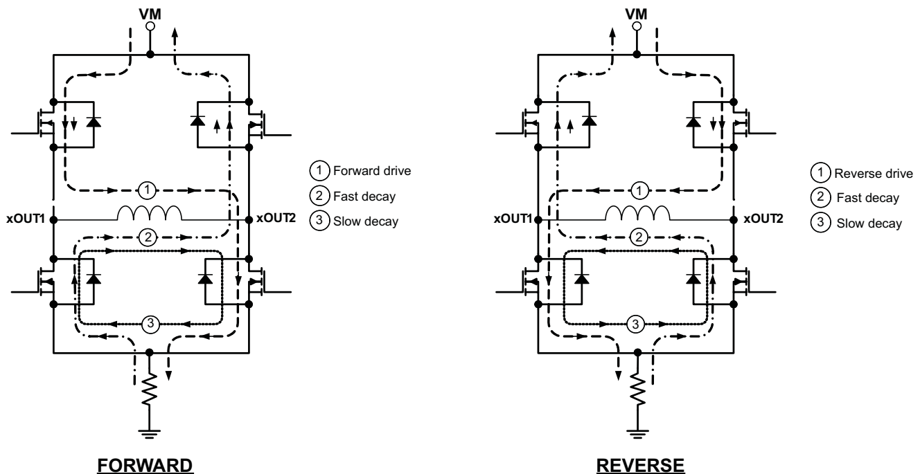
Figure 6. Drive and Decay Modes
